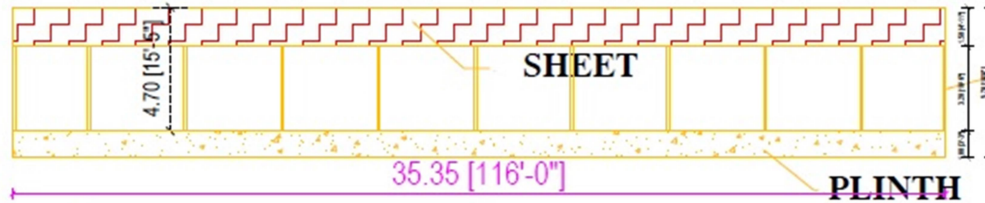
SECTION X-X
