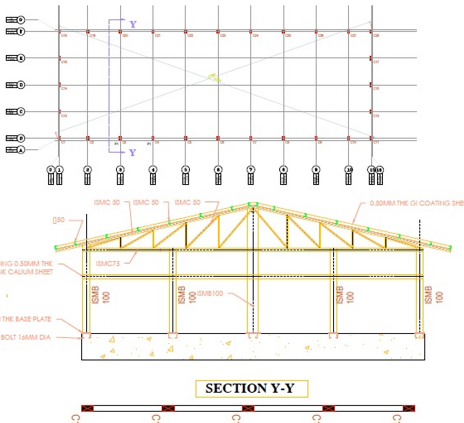
SECTION Y-Y STEEL STRUCTURAL SECTION MACHINERY UNIT SHED
