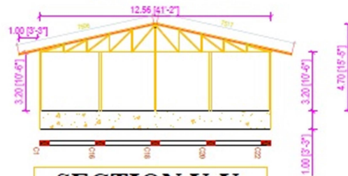
SECTION Y-Y
